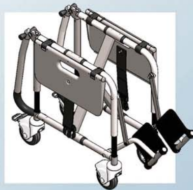
Two part movement for ease of folding. (Shown without seat and backrest)
